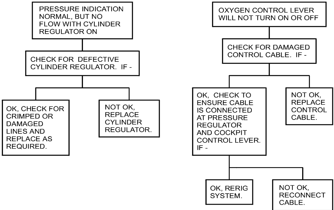
Figure 101 : Sheet 2 : Oxygen System Troubleshooting Chart
